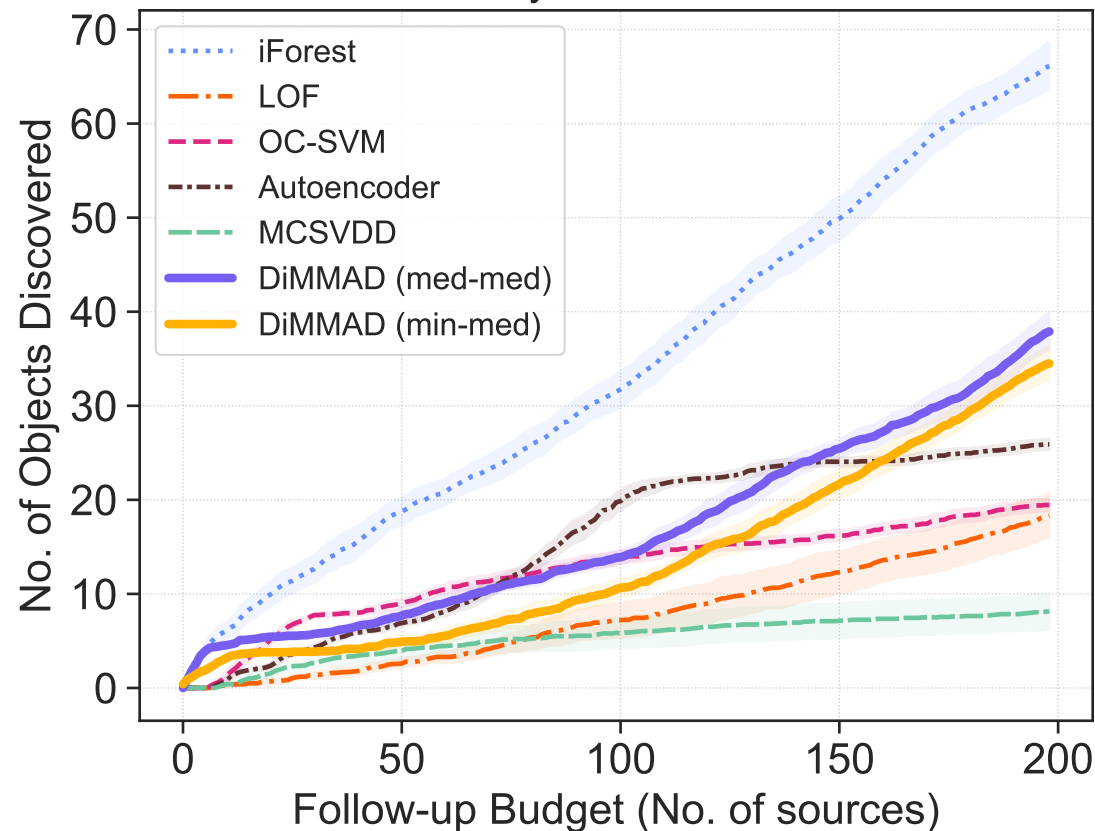
Anomaly: PISN-MOSFIT
